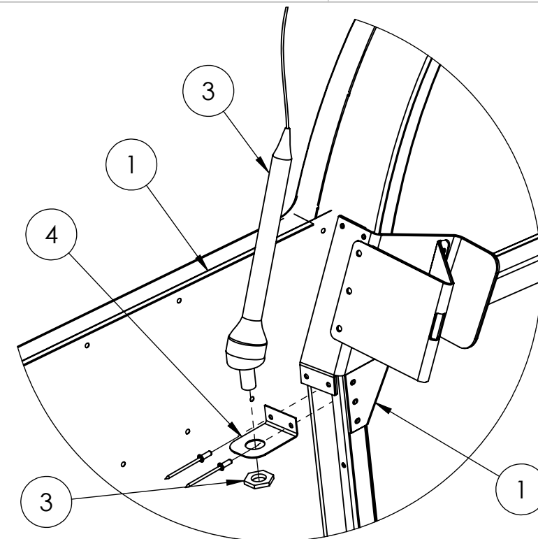
EXPLODED VIEW
