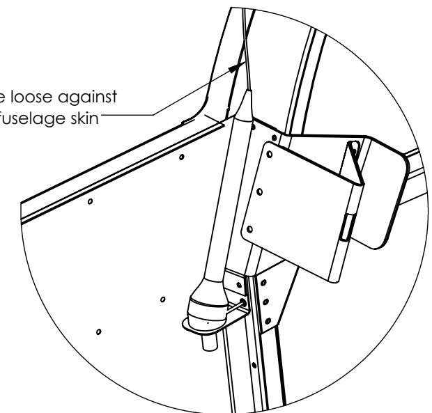
ASSEMBLED VIEW (DETAIL A)
