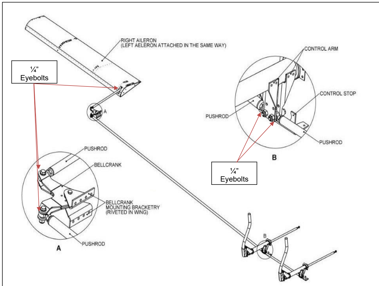
Figure 7: Aileron Controls
