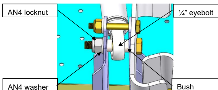
Figure 6: 1/4" eyebolt rudder pedal assembly
