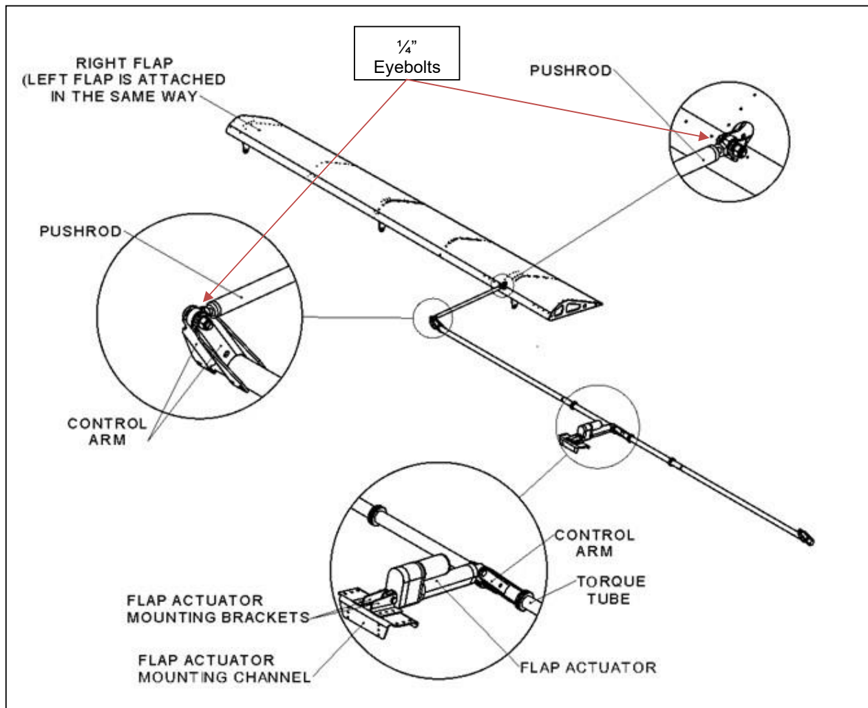
Figure 16: Flap Controls
