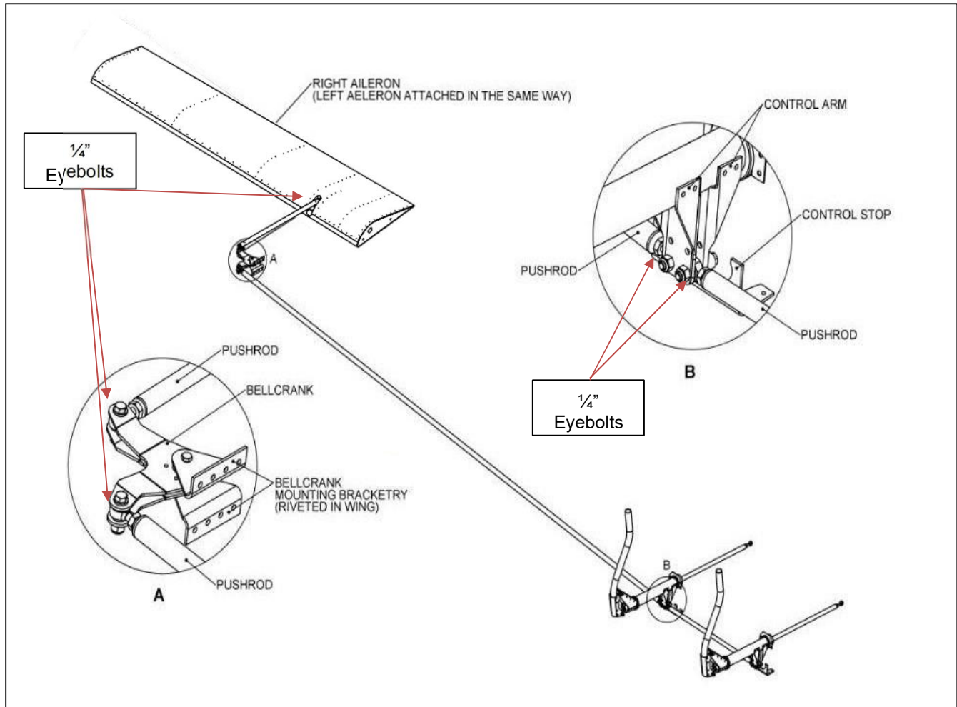
Figure 11: Aileron Controls
