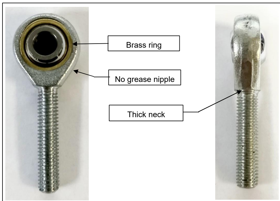
Figure 2: Type 2 Eyebolt
