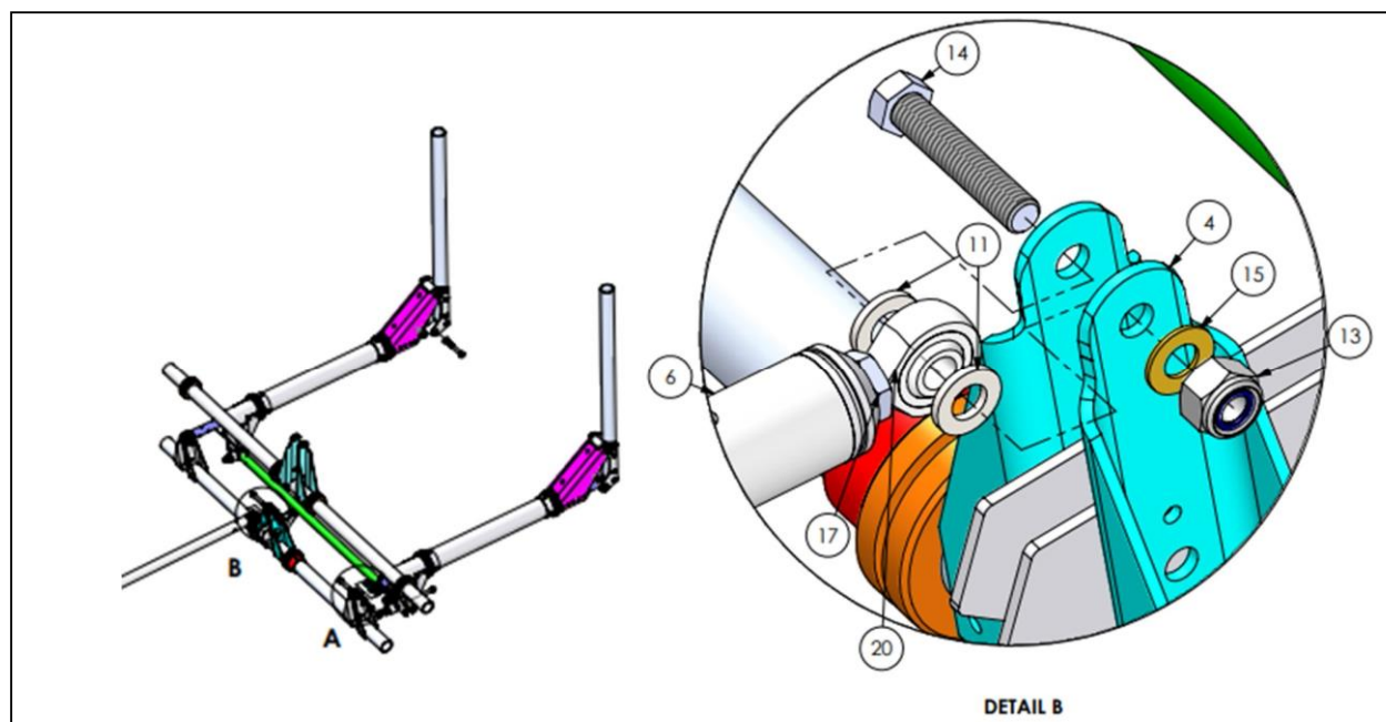
Figure 25: Eyebolt assembly, Detail B
