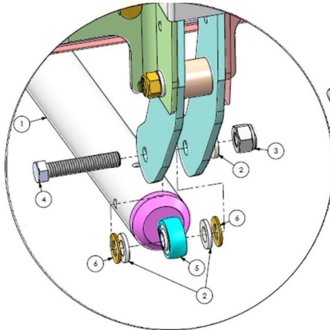
Figure 31: Detail G, exploded view
